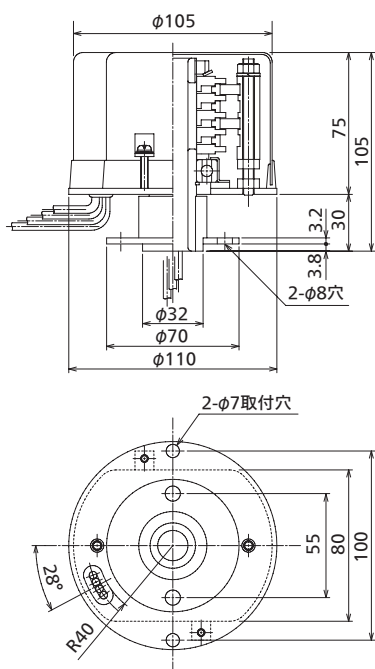
SR5013: AC (DC) 250V 13P15A
