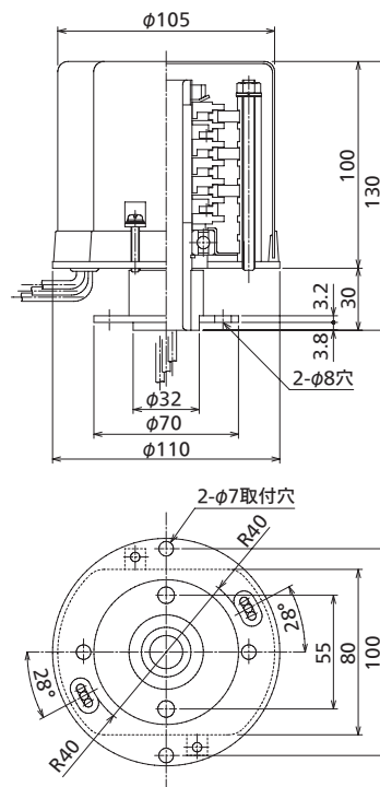
SR5006: AC (DC) 250V 6P15A
