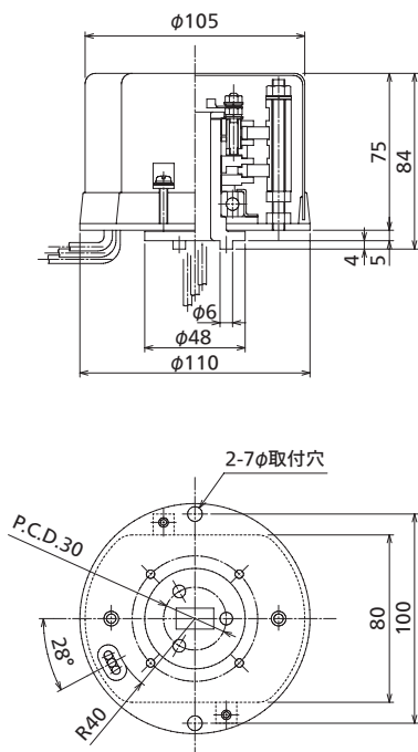
SR5010: AC (DC) 250V 10P15A
